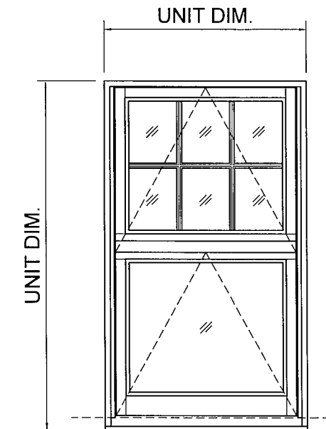
EXTERIOR ELEVATION OF SERIES 4000 IN-LINE FOLD-UP OUT WINDOW UNIT AT COUNTER
